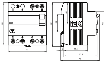
Figure 2 – Overall and installation dimensions of four-polar VDs
