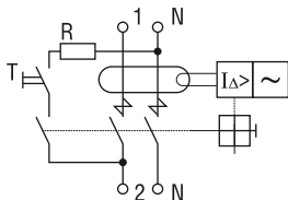
Figure 3 – Electric schematic diagram of two-polar VDs
