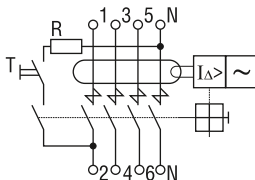
Figure 4 – Electric schematic diagram of four-polar VDs
