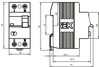
Figure 1 – Overall and installation dimensions of two-polar VDs
