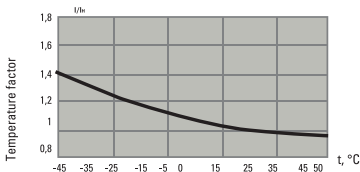
Figure 1 – Derating factor depending on ambient temperature
