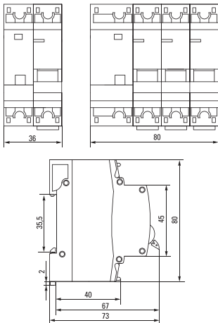
Figure 2 – Overall dimensions
